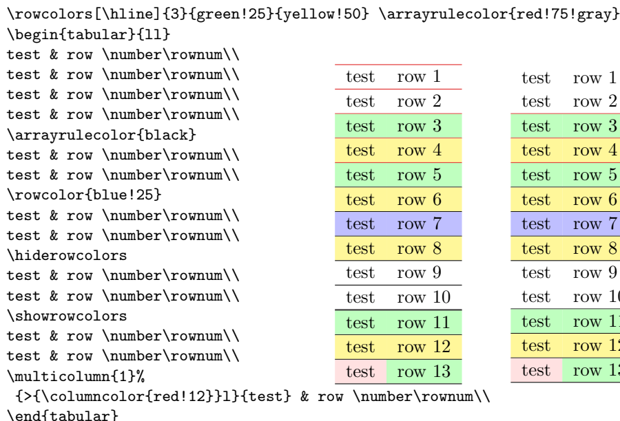
Figure 10: Alternating row colors in tables: \rowcolors vs. \rowcolors*
